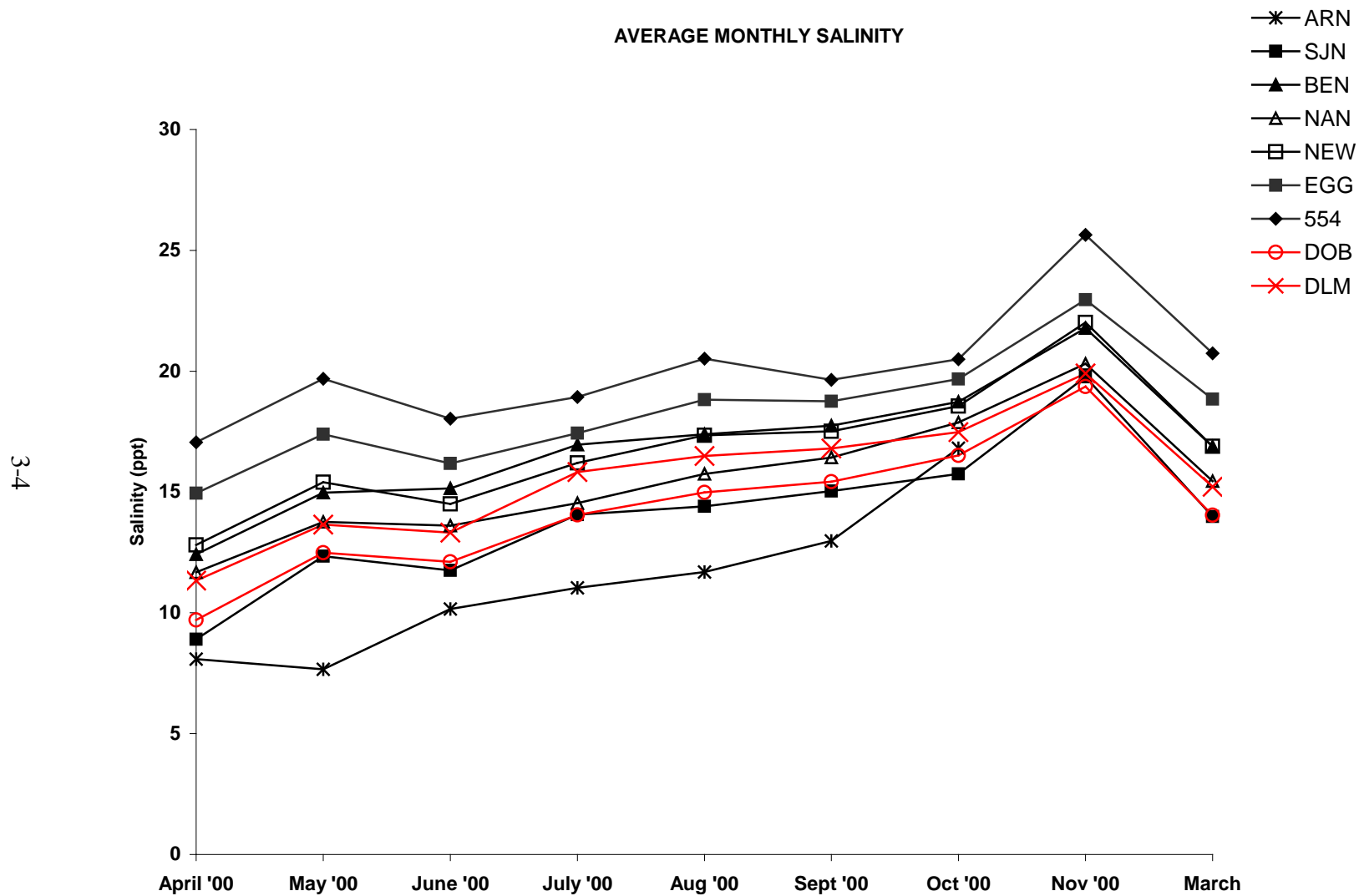
Figure 3-3. Monthly salinity measured at the nine oyster bed monitoring stations in Delaware Bay
