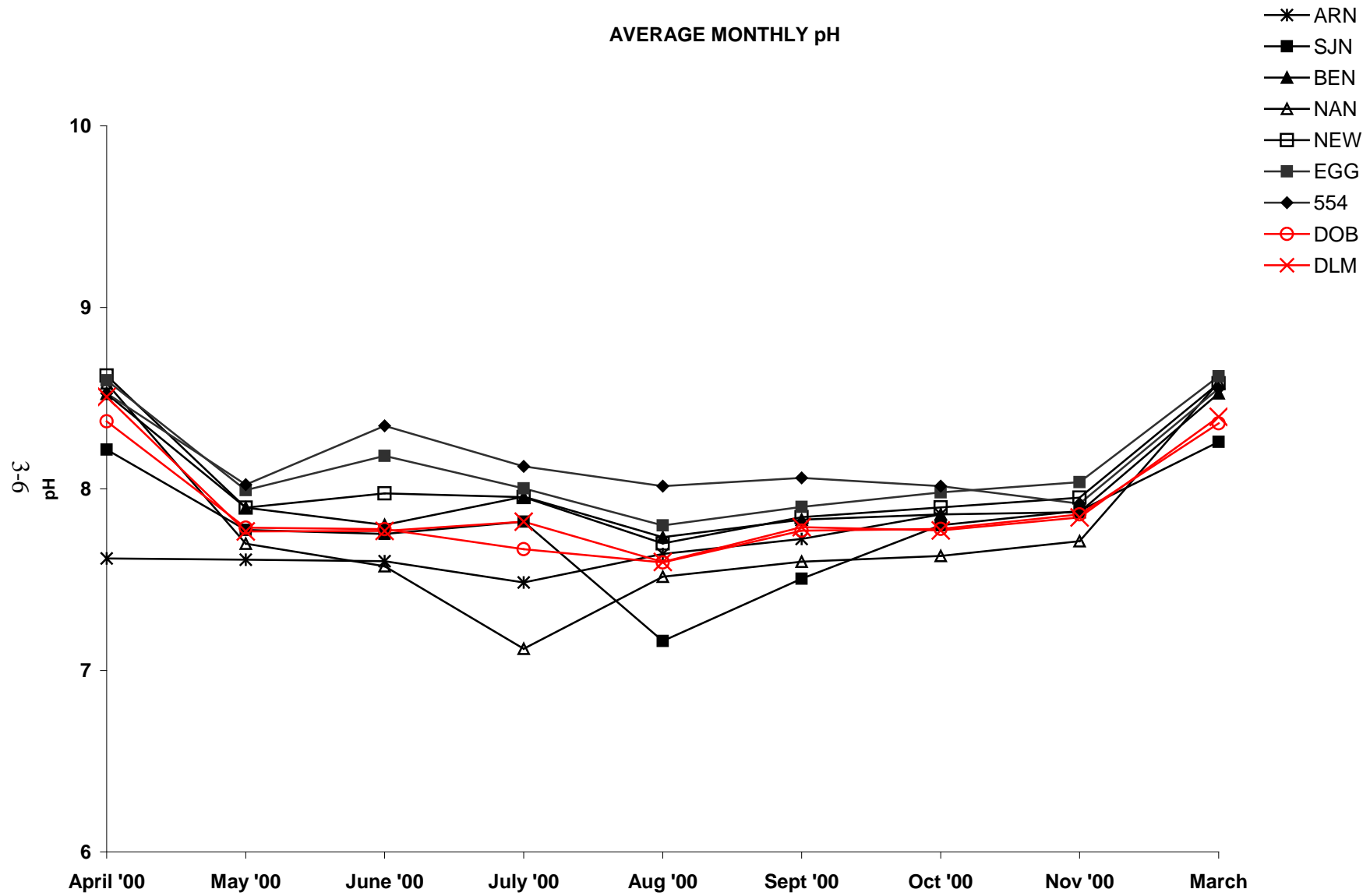
Figure 3-5. Monthly pH measured at the nine oyster bed monitoring stations in Delaware Bay
