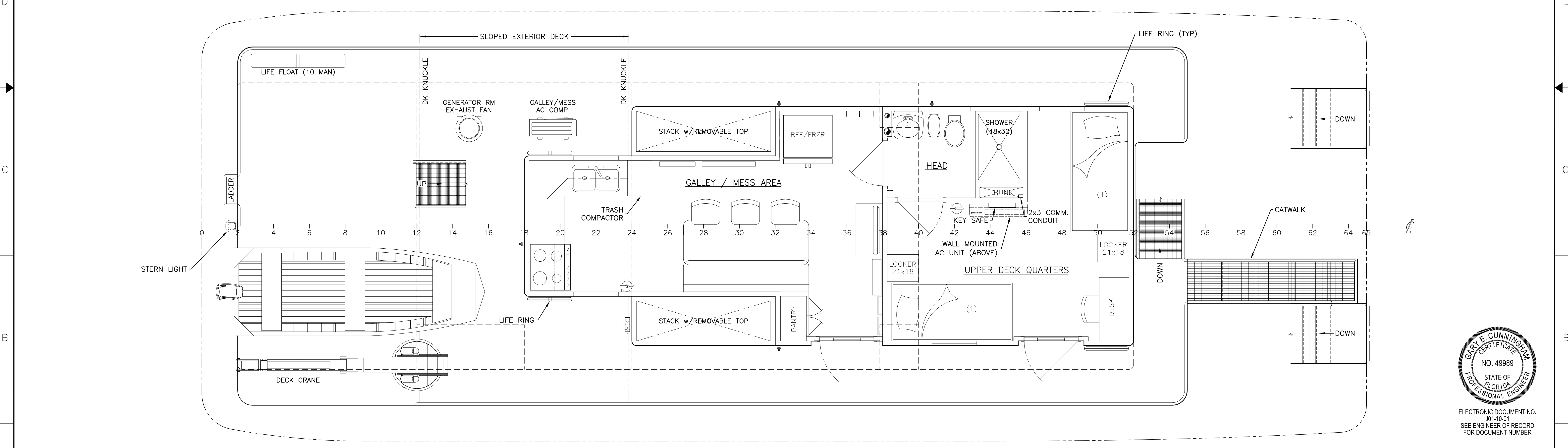
UPPER DECK PLAN
