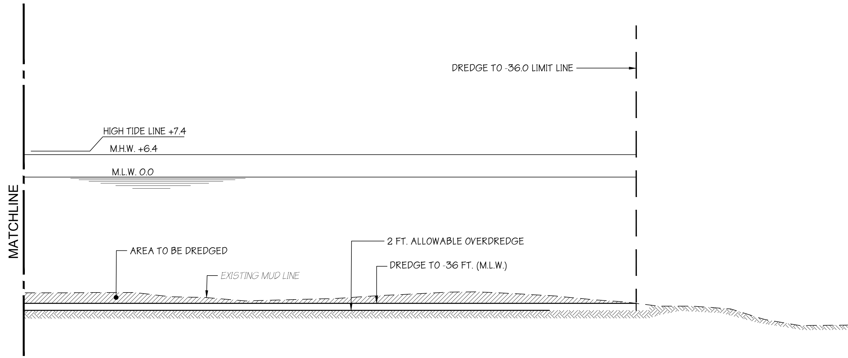
(SECTION LOOKING DOWNRIVER) DREDGE SECTION SCALE 1/16" = 1'-0"
