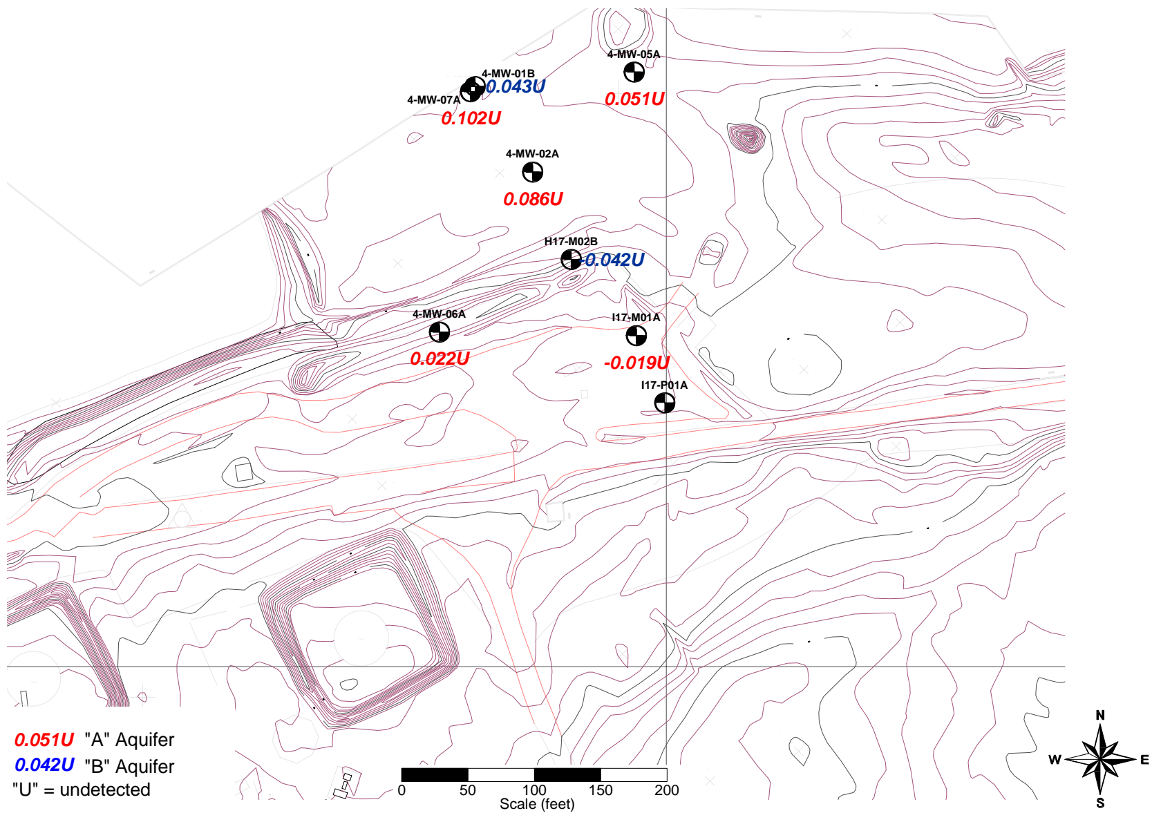
Figure H-4 Thorium-230 Contour Map - "A" and "B" Aquifers AOC 4
