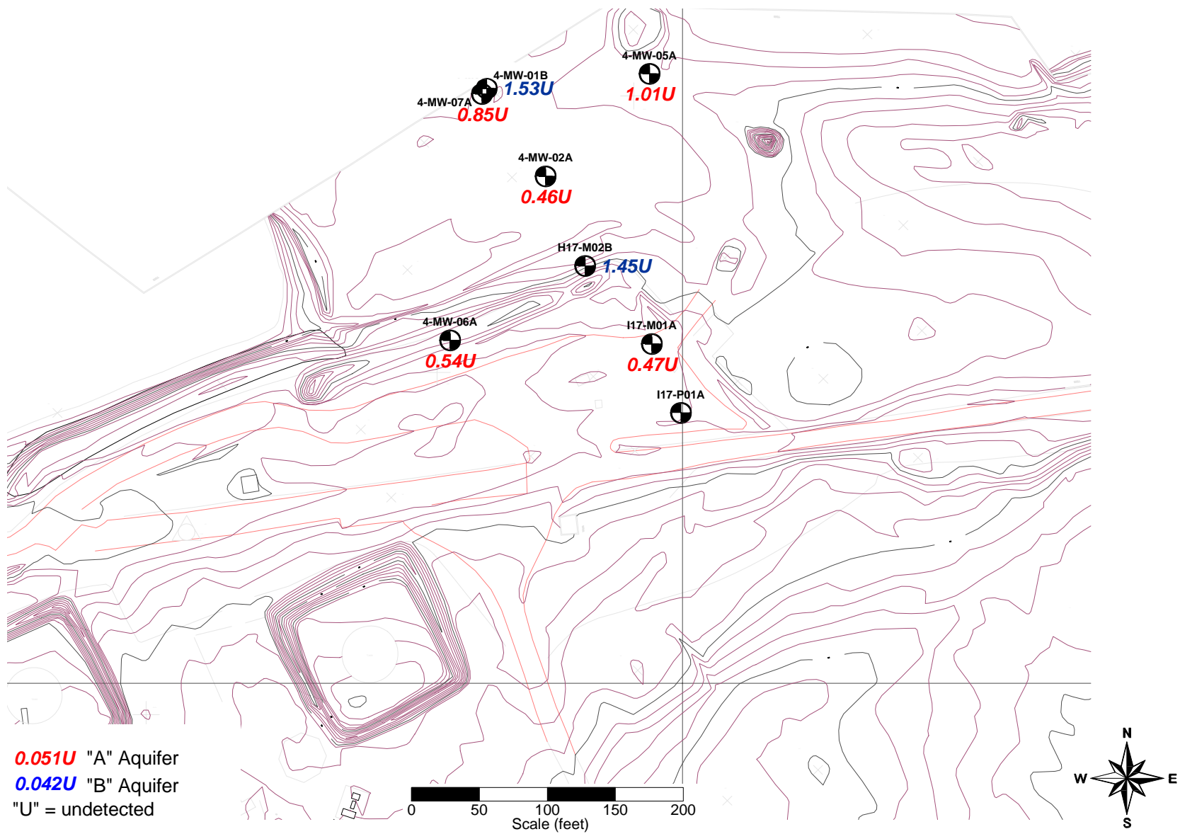
Figure H-3 Ra-226 + Ra-228 Contour Map - "A" and "B" Aquifers AOC 4
