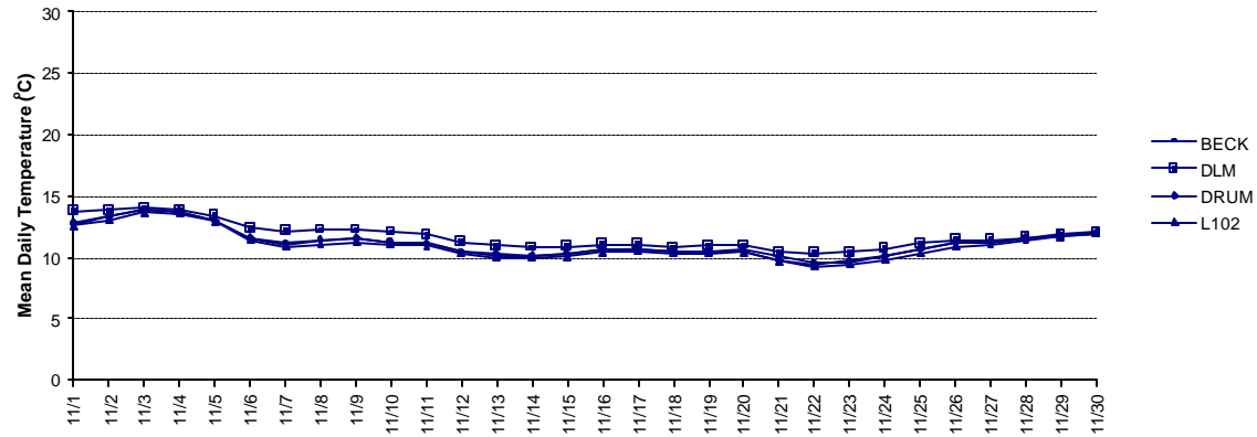
Figure A-1g. Mean daily water temperature measured during November 2001 at Delaware Bay oyster beds, Becks Rock (BECK), Delaware Lower Middle (DLM), Drum Bed (DRUM), and Lease Bed 102 (L102).
