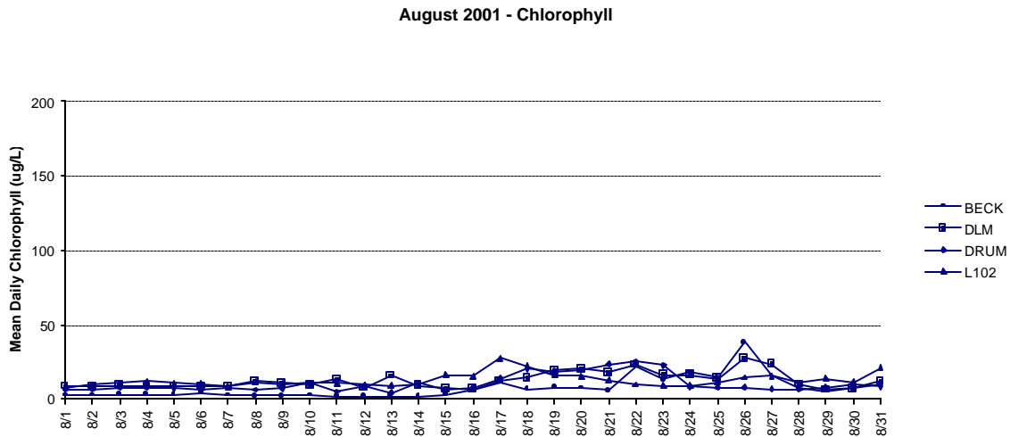
Figure A-7d. Mean daily chlorophyll measured during August 2001 at Delaware Bay oyster beds, Becks Rock (BECK), Delaware Lower Middle (DLM), Drum Bed (DRUM), and Lease Bed 102 (L102).
