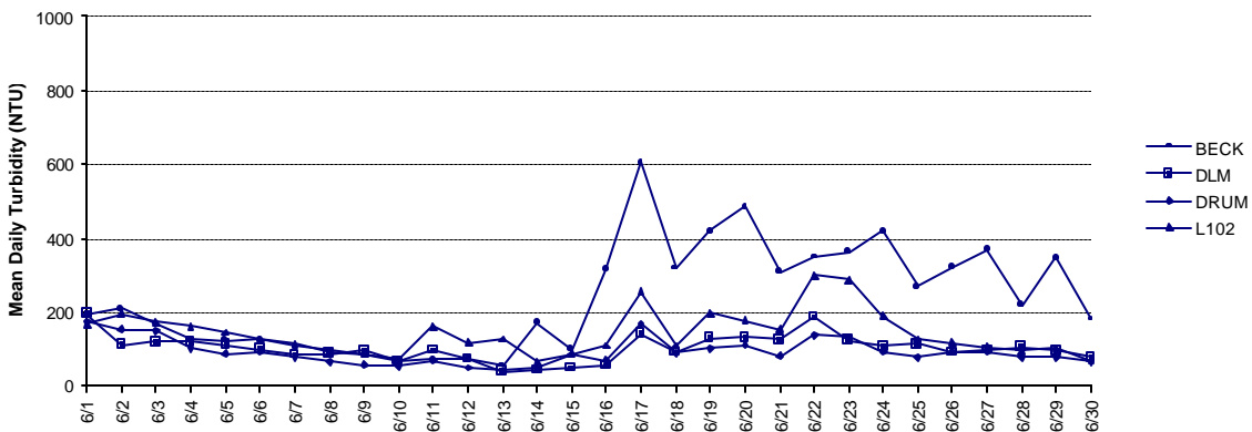
June 2001 - Turbidity
