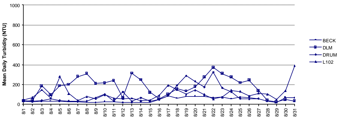
August 2001 - Turbidity
