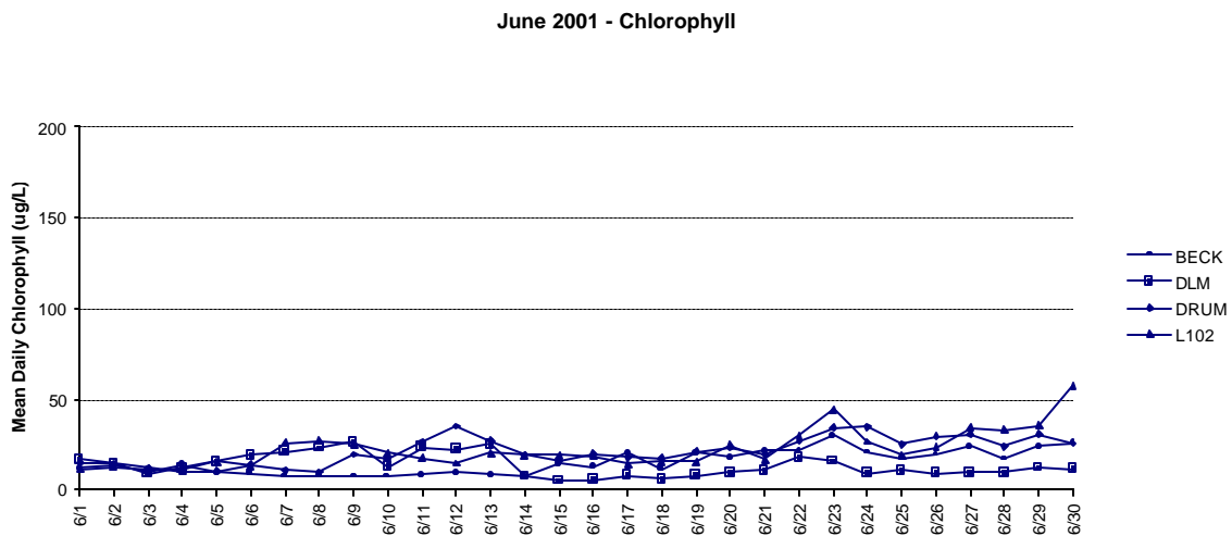
Figure A-7b. Mean daily chlorophyll measured during June 2001 at Delaware Bay oyster beds, Becks Rock (BECK), Delaware Lower Middle (DLM), Drum Bed (DRUM), and Lease Bed 102 (L102).
