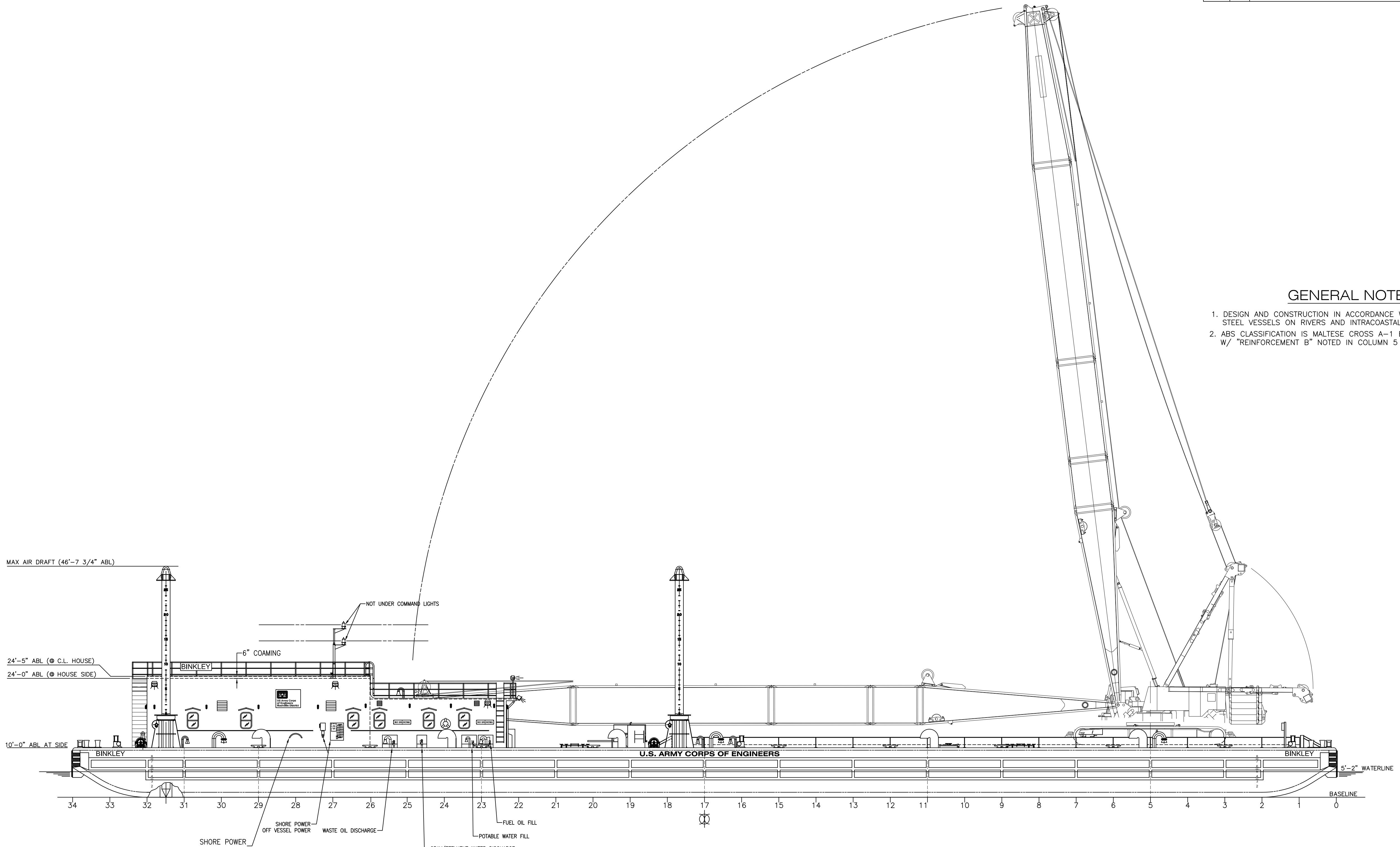
OUTBOARD PROFILE
