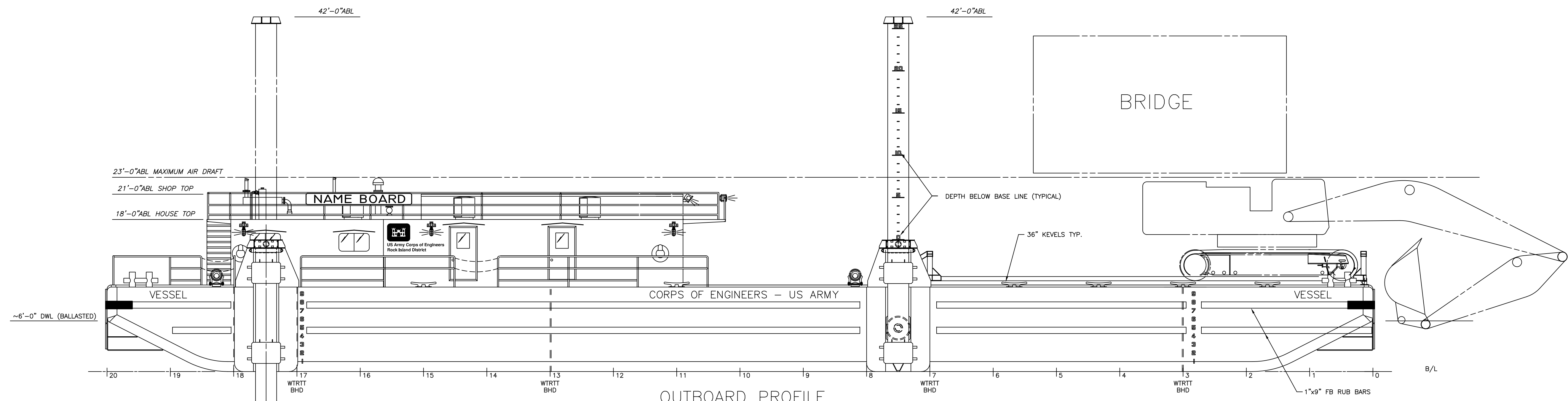
OUTBOARD PROFILE
