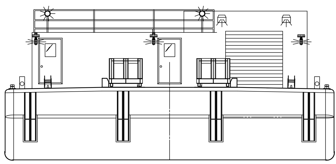
END (BOW) VIEW SPUDS NOT SHOWN
