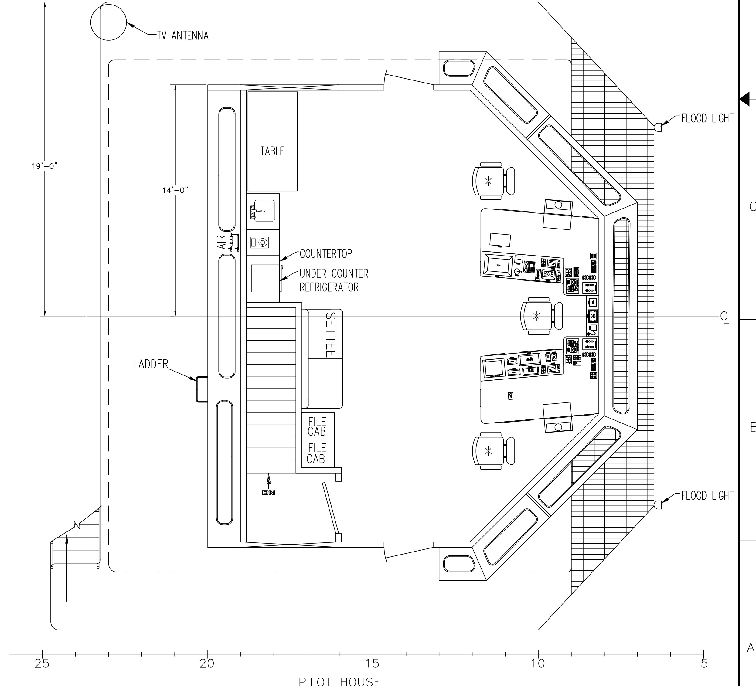
PILOT HOUSE TOP PLAN
