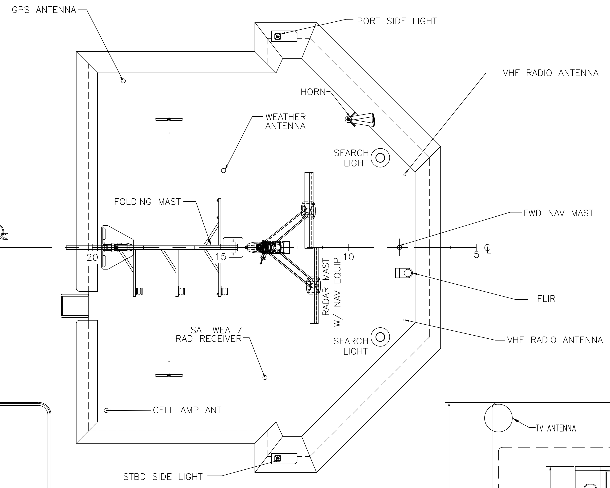
PILOT HOUSE TOP PLAN
