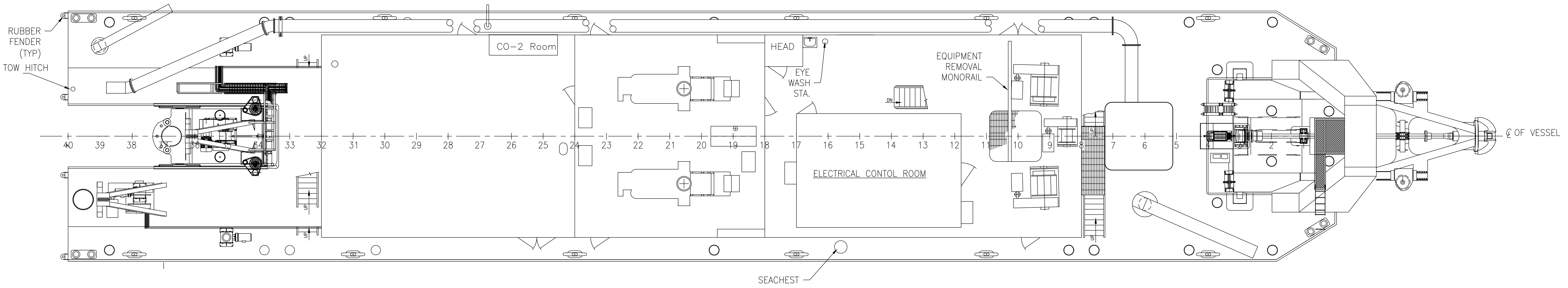
MAIN DECK PLAN
