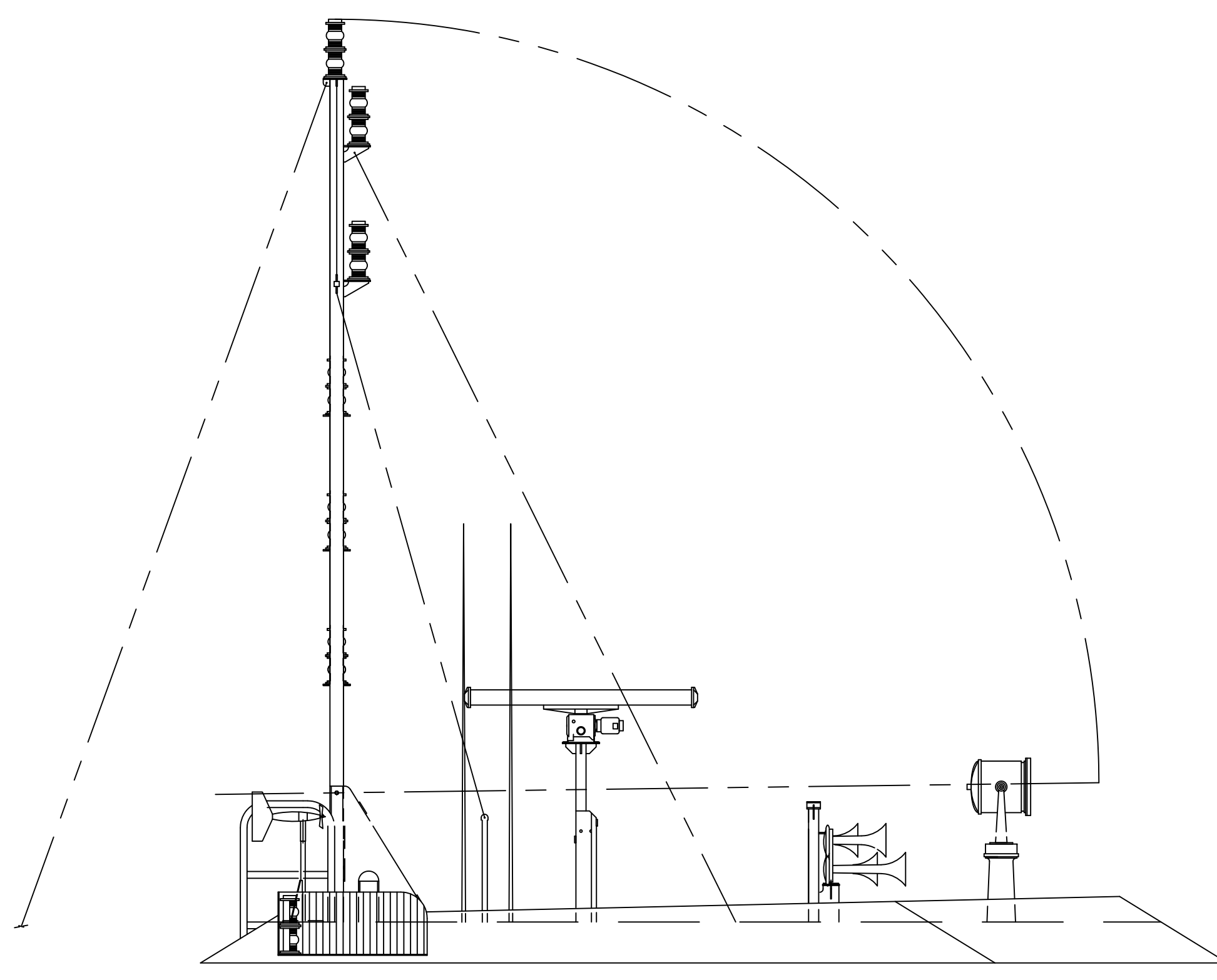
PILOT HOUSE TOP WITH FOLDING MAST
