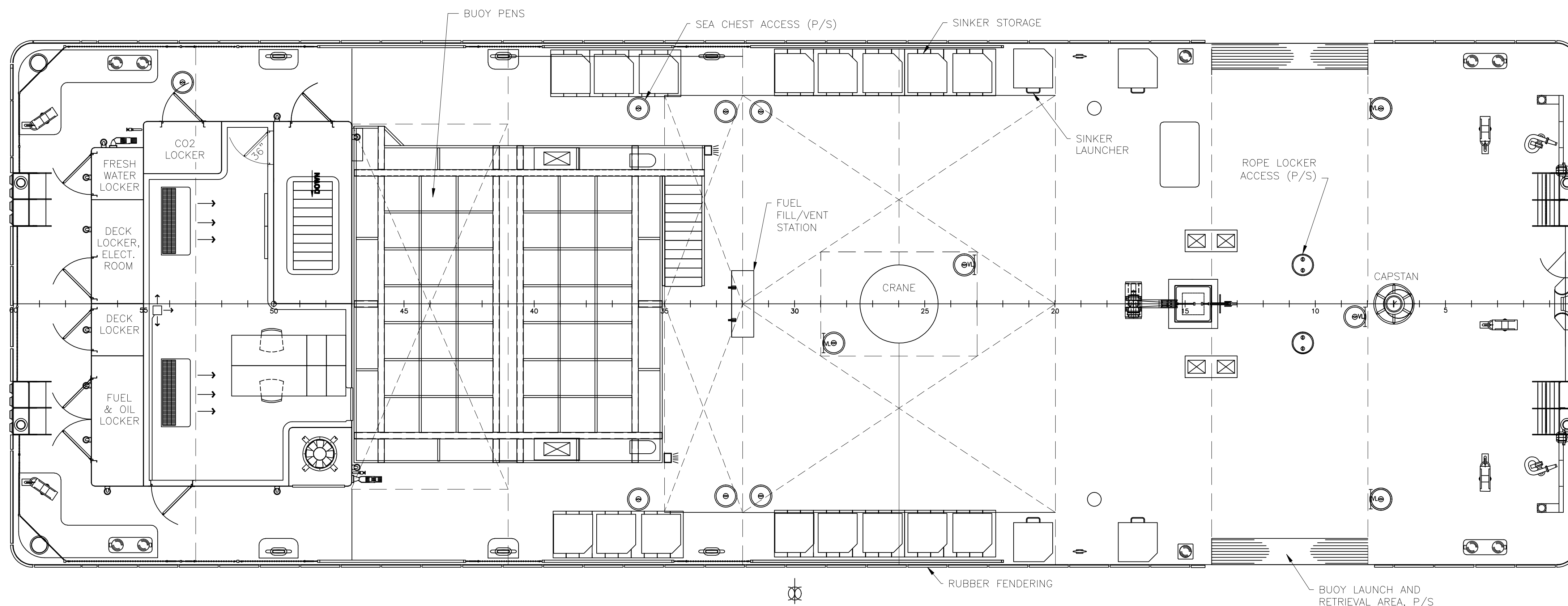
PLAN VIEW MAIN DECK ARRANGEMENT
