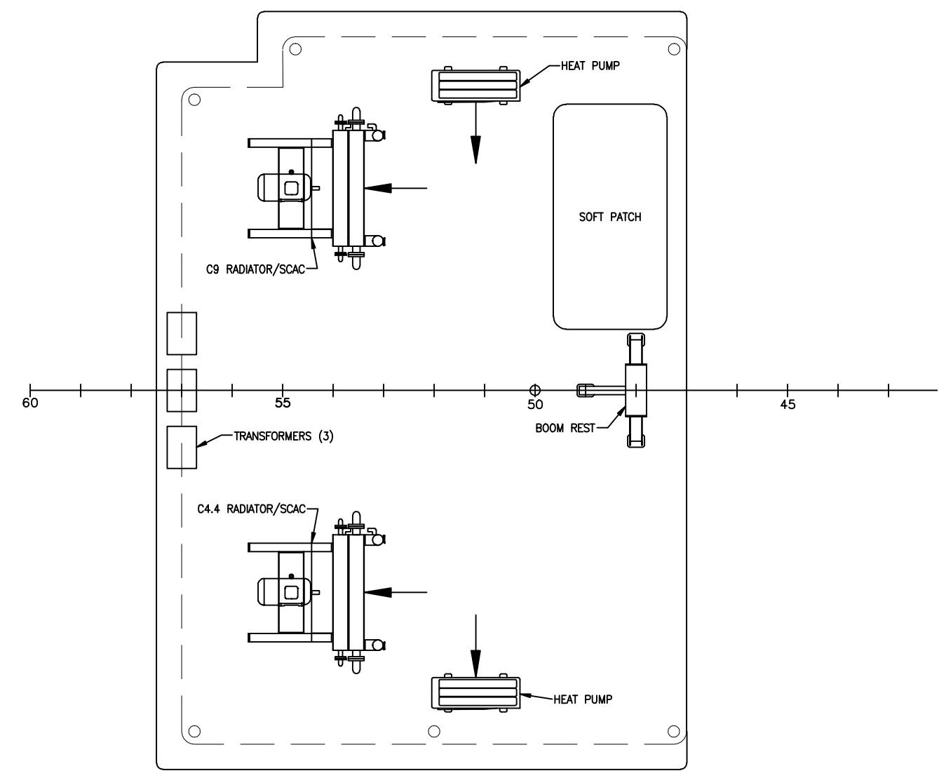
DECKHOUSE TOP
