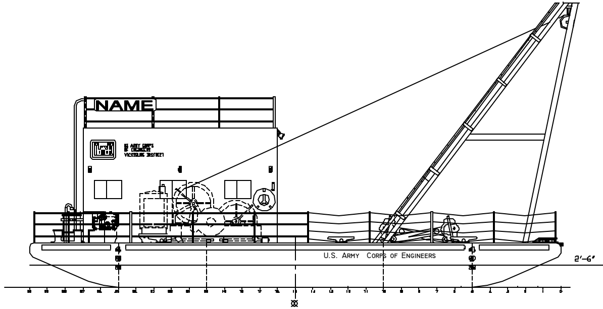
OUTBOARD PROFILE
