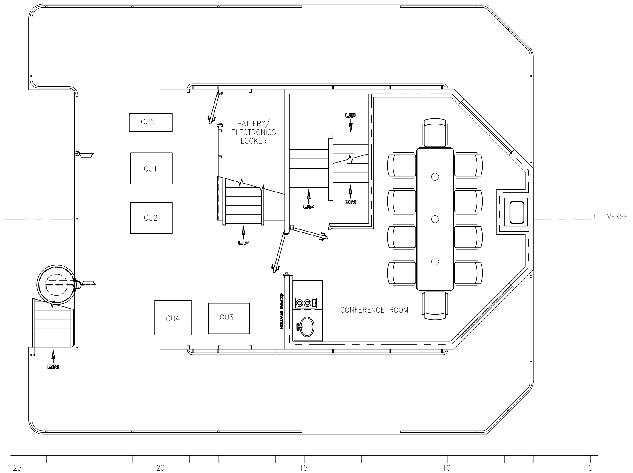
PLAN @ PLENUM DECK
