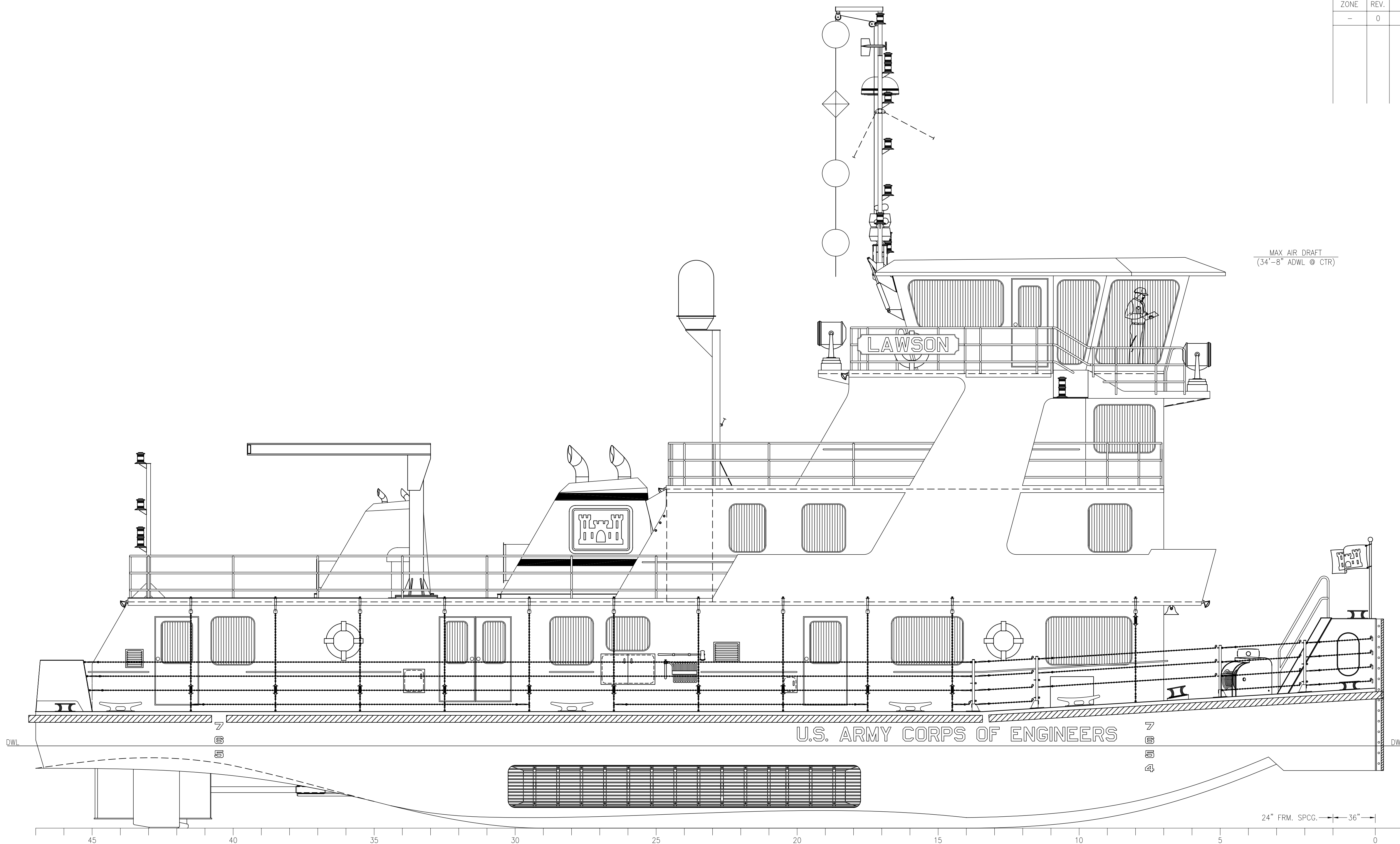
OUTBOARD PROFILE LOOKING TO PORT
