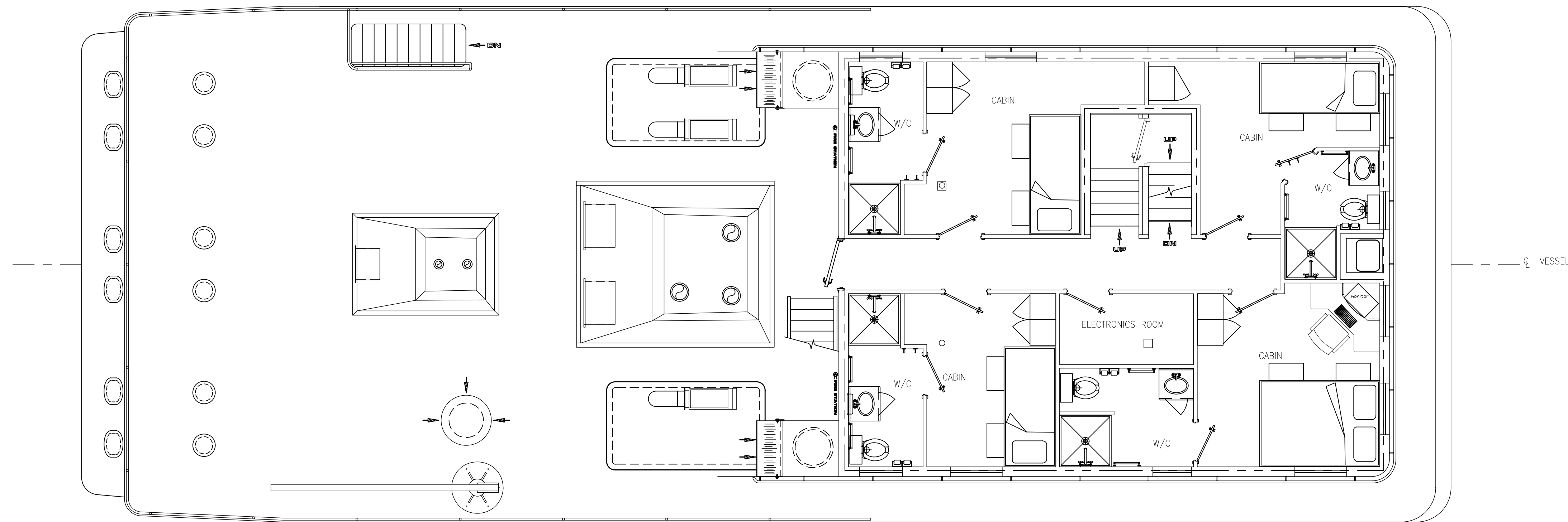
PLAN @ UPPER DECK
