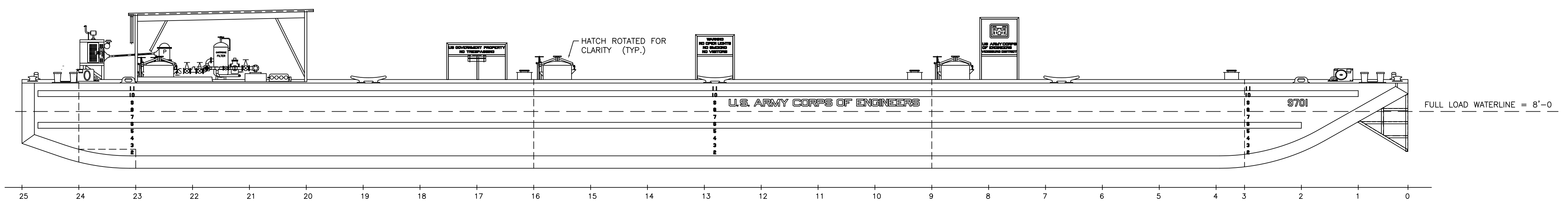
OUTBOARD PROFILE
