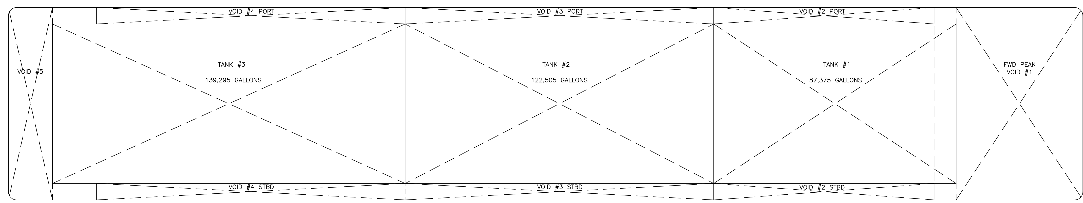
TANK ARRANGEMENT
