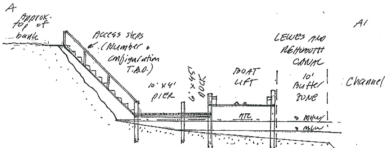
Figure 8. Plan view and cross-section sketches of proposed project. Sketches for permit application purposes only.
